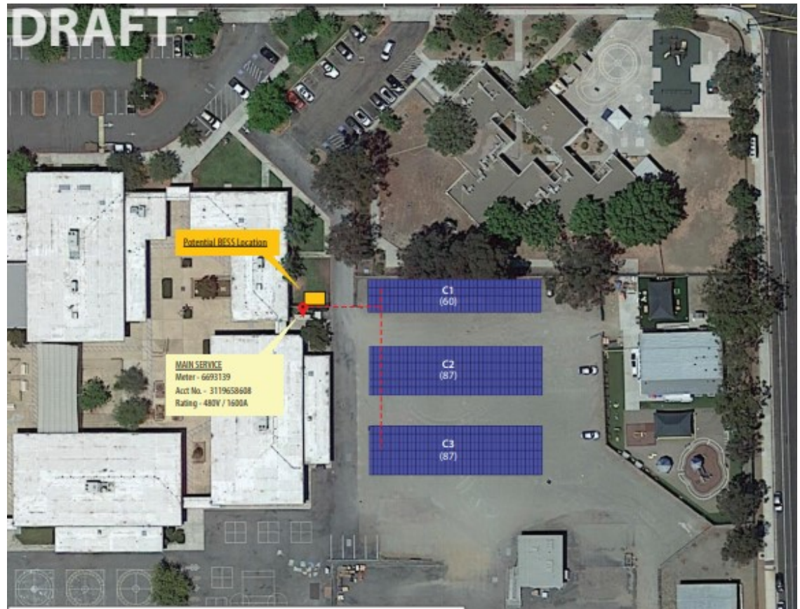
Proposed solar array placement
