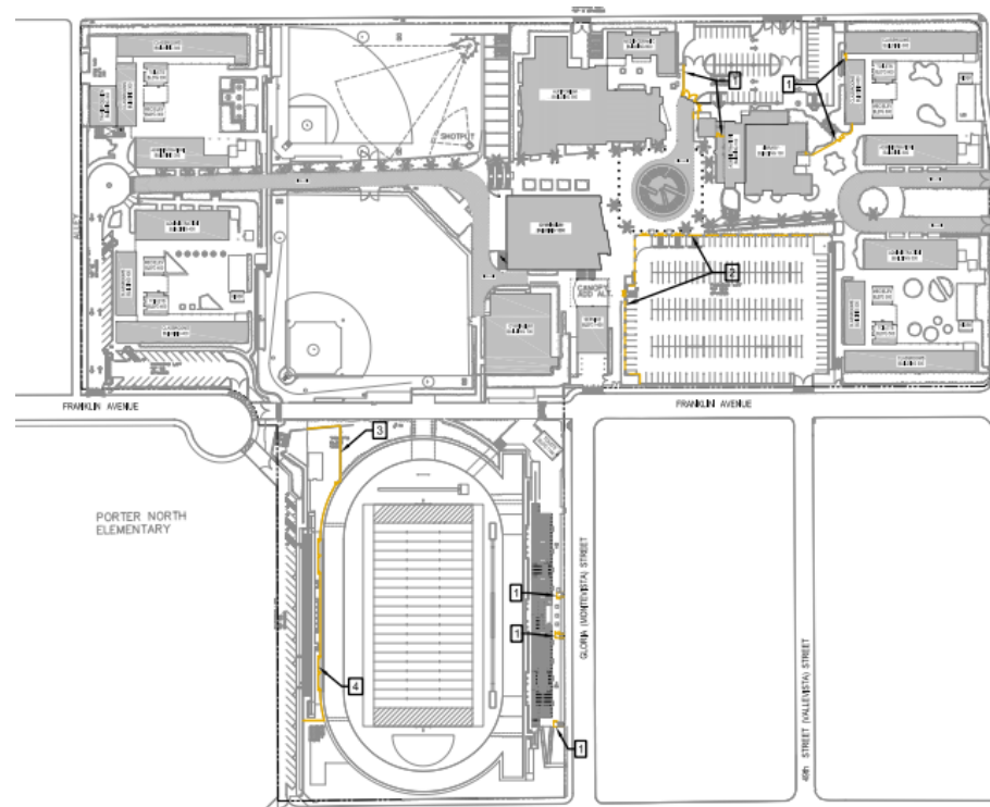
Site plan of Fencing Project
